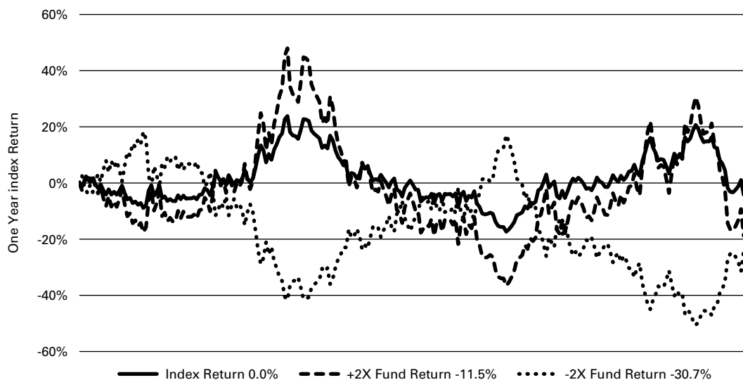
One-Year Simulation; Benchmark Flat (0%) (Annualized Benchmark Volatility 35%)
